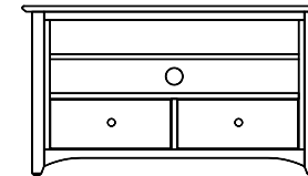
TV UNIT WITH DRAWERS H: 600 W: 1080 D: 425
