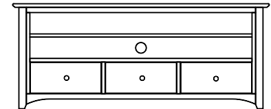
LARGE TV UNIT WITH DRAWER H: 600 W: 1450 D: 425
