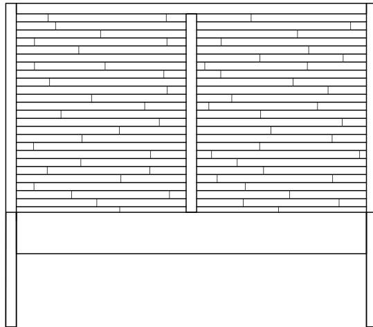
4'6" LOW FOOT END SLEIGH BED H: 1240 W: 1420 D: 2150
