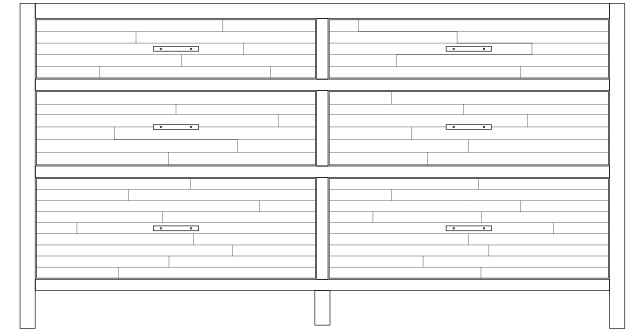
3 + 3 WIDE CHEST H: 860 W: 1600 D: 450
