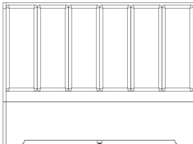
4' 6" LOW FOOT END BED H: 1200 W: 1484 D: 2020
